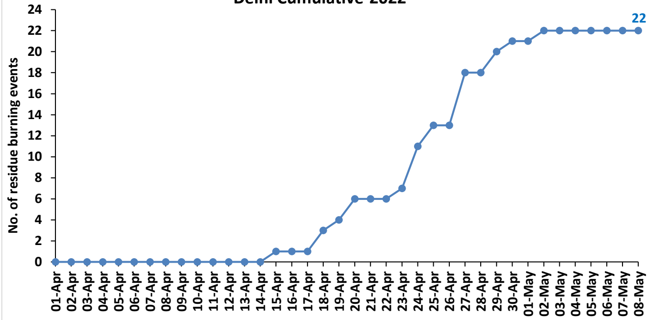
Delhi Cumulative-2022
