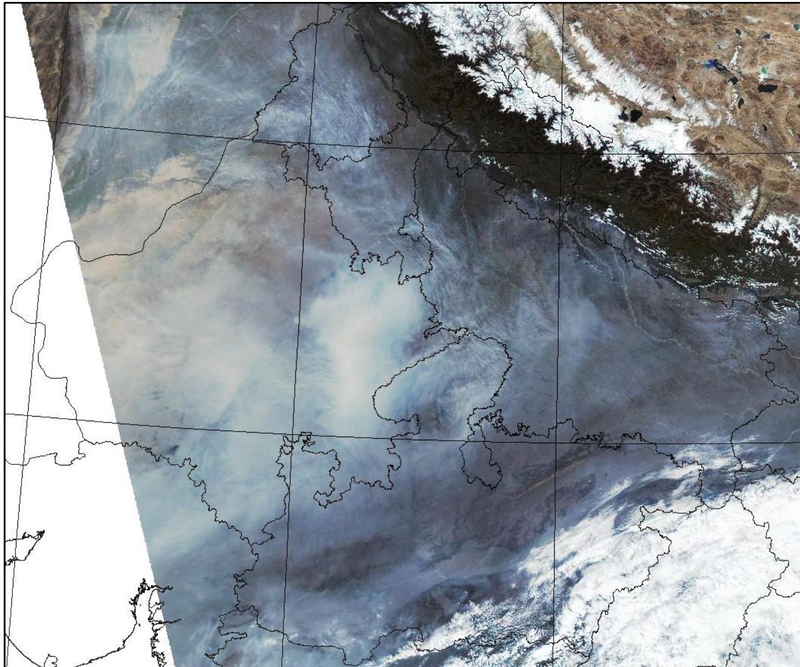
AQUA (MODIS) Satellite image (TCC) of North and Central India Acquired on 13-Nov-2021 at 13:11:00 IST by IARI Ground Station
