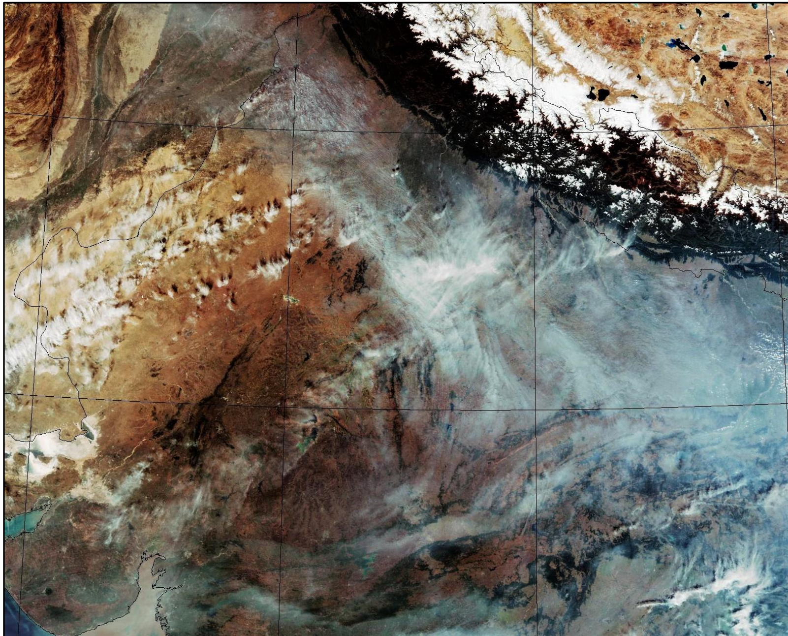
SNPP (VIIRS) Satellite image (TCC) of North and Central India Acquired on 10-Nov-2021 at 13:33:00 IST by IARI Ground Station
