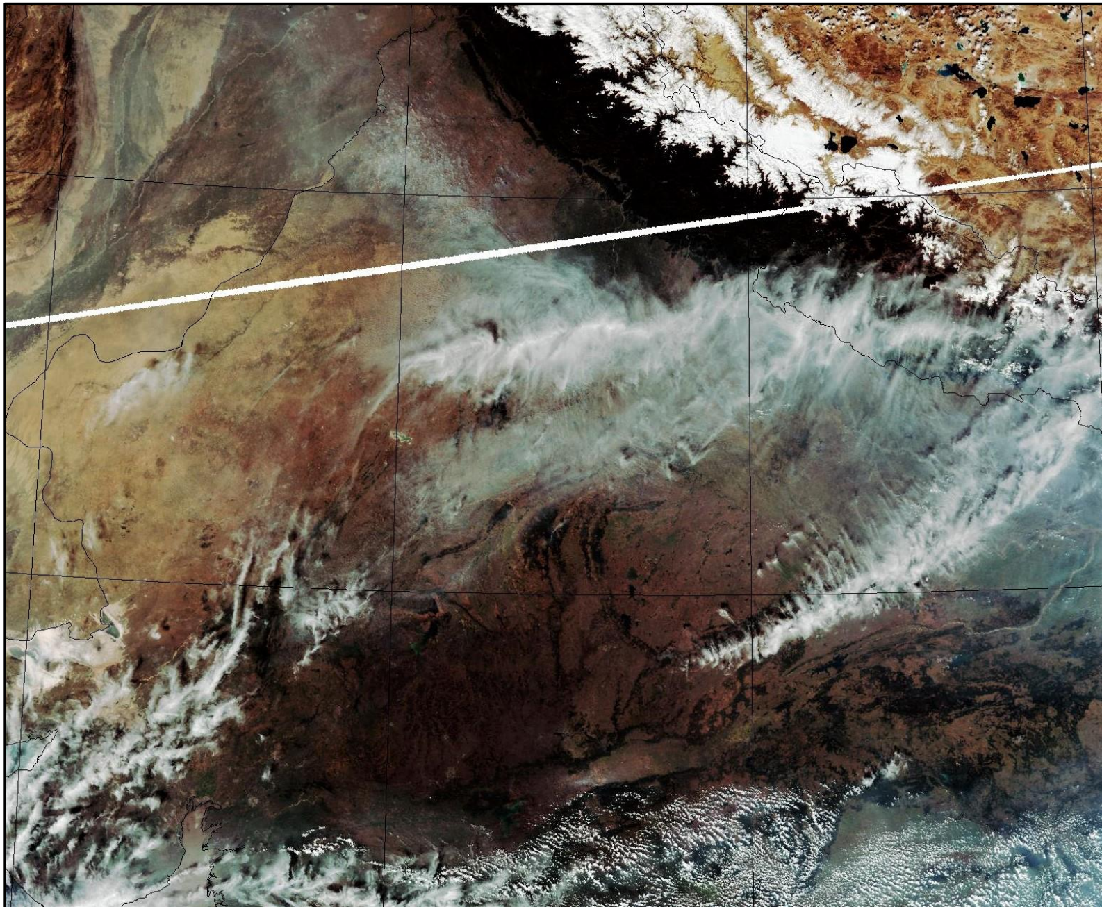
SNPP (VIIRS) Satellite image (TCC) of North and Central India Acquired on 05-Nov-2021 at 13:26:00 IST by IARI Ground Station
