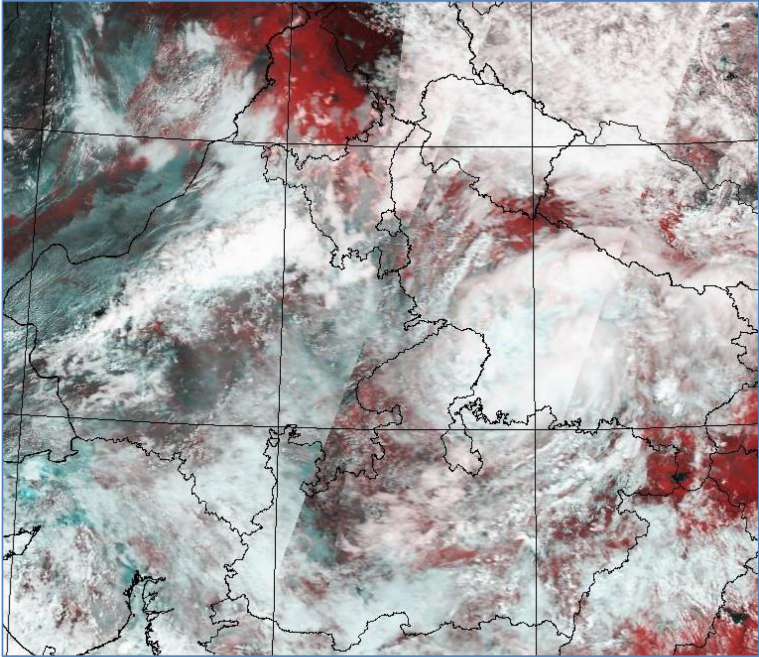
METOP-1 (VHRR) Satellite image (FCC) of North and Central India Acquired on 24-Sep-2021 at 10:46:05 IST by IARI Ground Station
