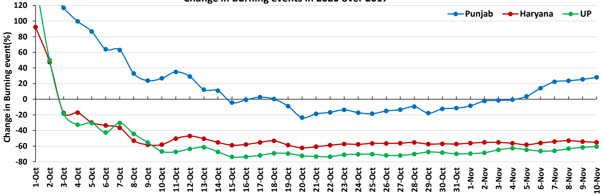
Change in Burning events in 2020 over 2017
