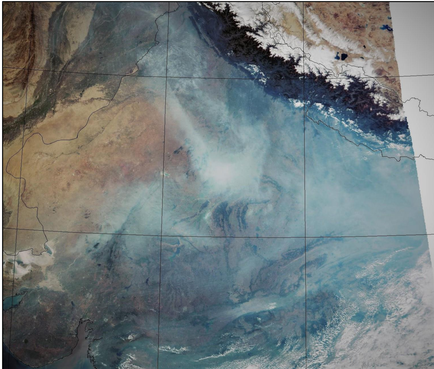
SNPP (VIIRS) Satellite image (TCC) of North and Central India Acquired on 14-Nov-2021 at 13:58:00 IST by IARI Ground Station
