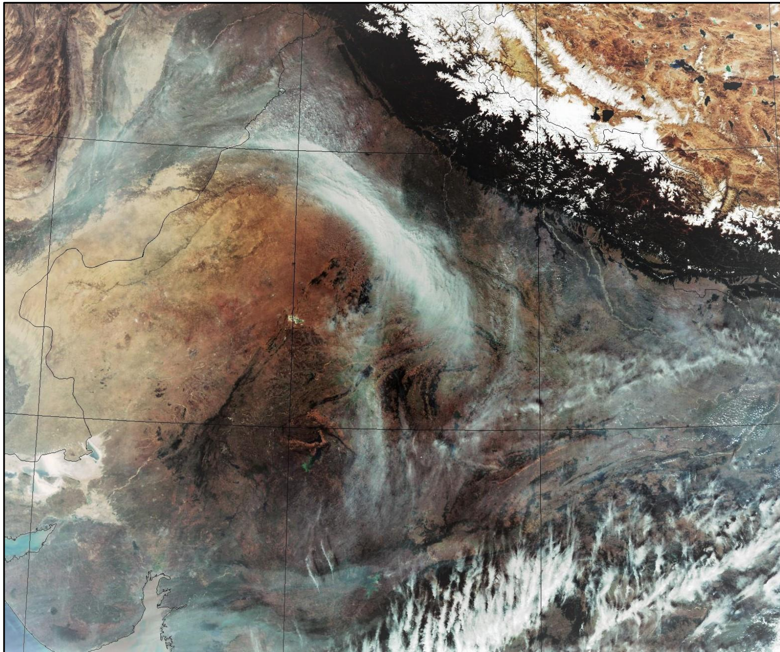
SNPP (VIIRS) Satellite image (TCC) of North and Central India Acquired on 11-Nov-2021 at 13:14:00 IST by IARI Ground Station
