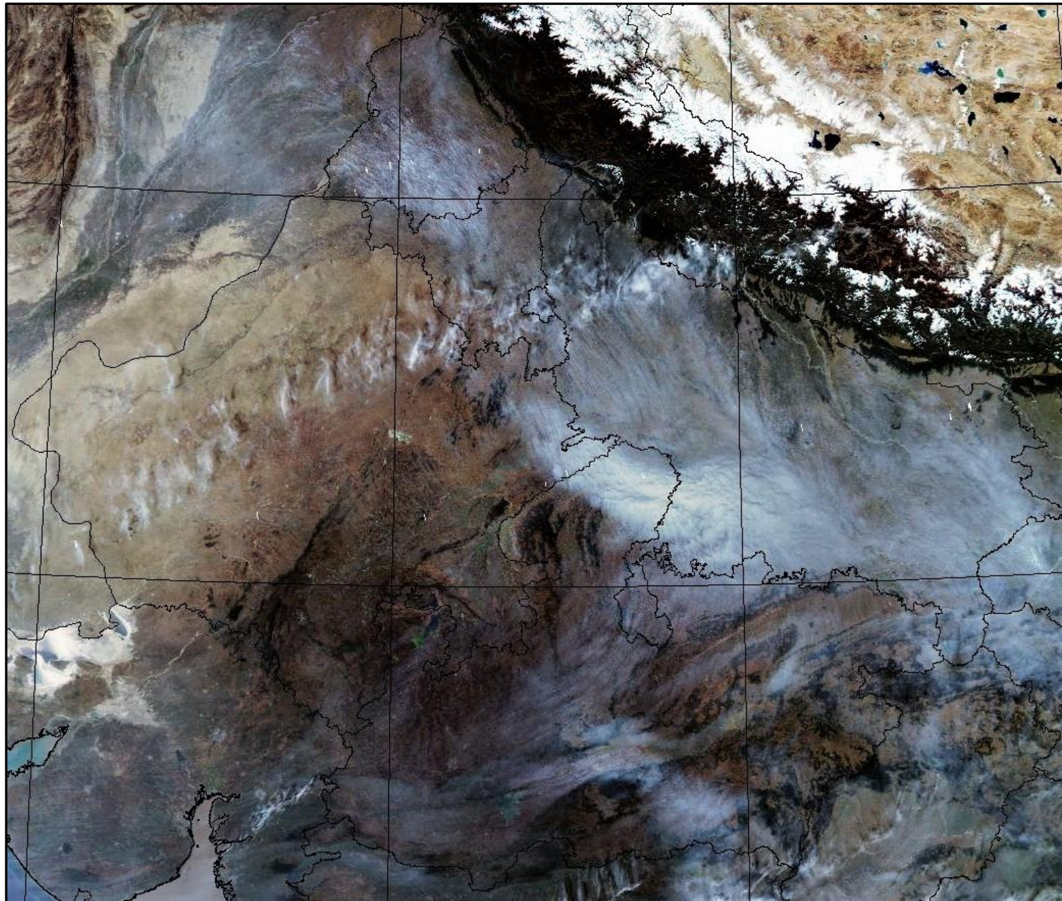
AQUA (MODIS) Satellite image (TCC) of North and Central India Acquired on 09-Nov-2021 at 13:35:00 IST by IARI Ground Station
