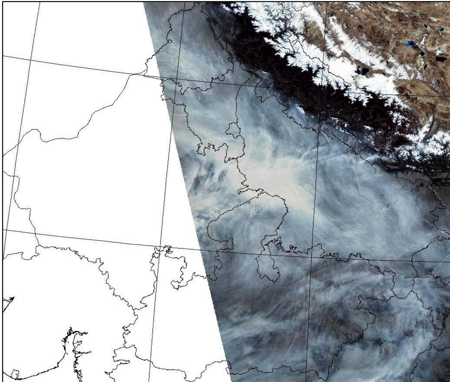
AQUA (MODIS) Satellite image (TCC) of North and Central India Acquired on 08-Nov-2021 at 12:53:00 IST by IARI Ground Station
