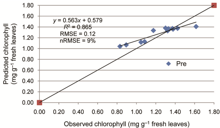
Figure 1. Observed and predicted chlorophyll content using the RGRcan model.
